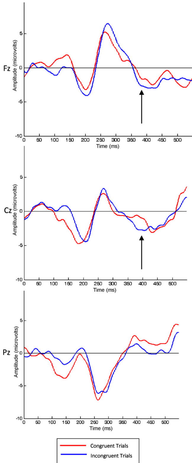
Fig. 2. N2 waveforms for congruent and incongruent trials.
