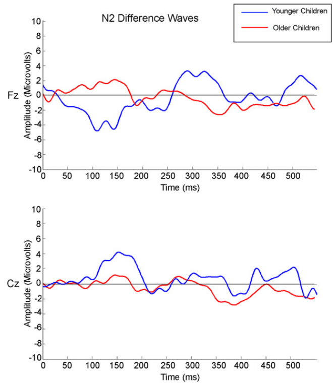
Fig. 3. N2 difference waveforms by age group.
